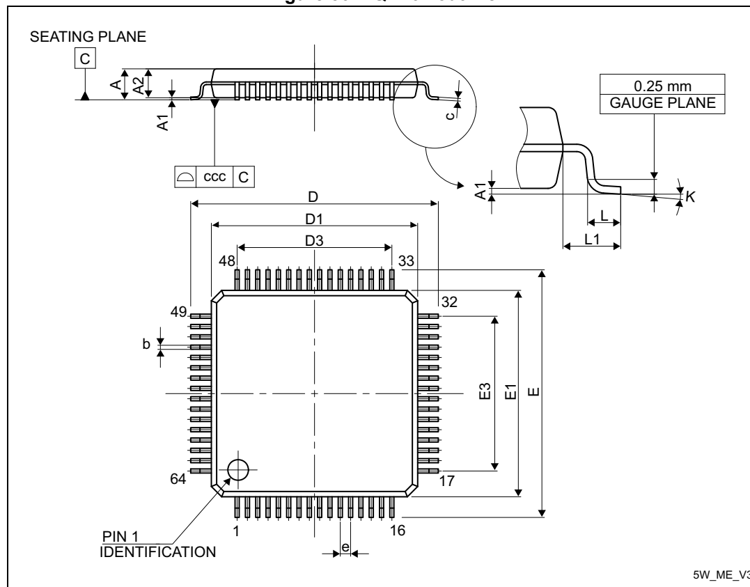
Figure 56. LQFP64 outline
